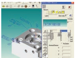
CAT 1000P Wizard defines GD&T on CAD file
