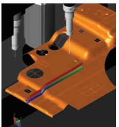
MCOSMOS Level 3 Virtual CMM Interface also used for scanning on CAD model
